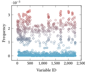
Figure 3: Distribution of propagation frequency.
