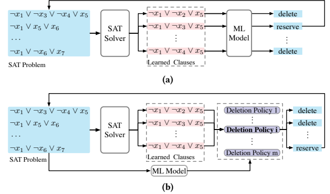
Figure 1: Two learning aided clause deletion mechanisms. (a) Evaluate learned clauses directly; (b) Evaluate clause deletion policies.
